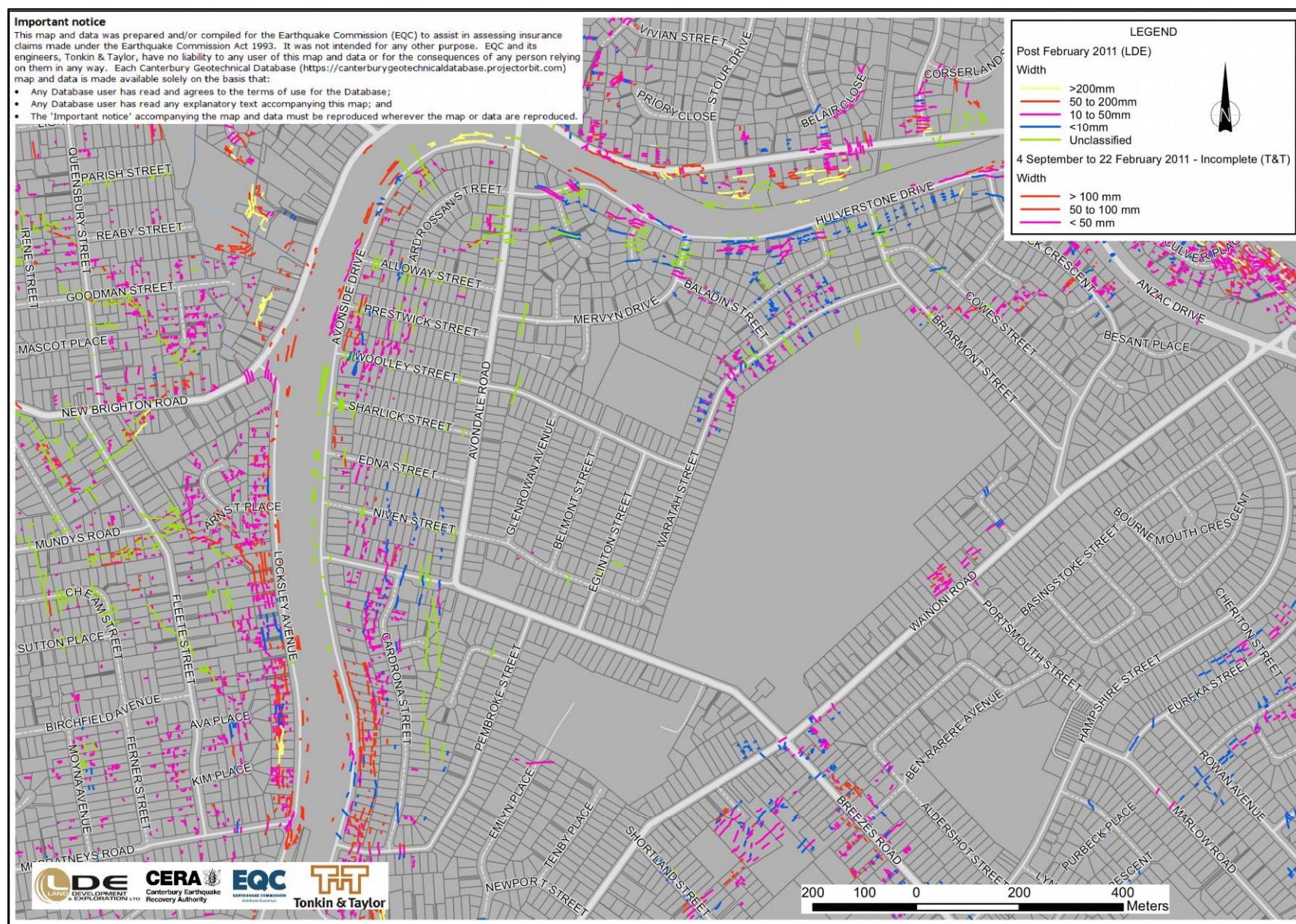
Figure 2 – Observed ground crack locations
