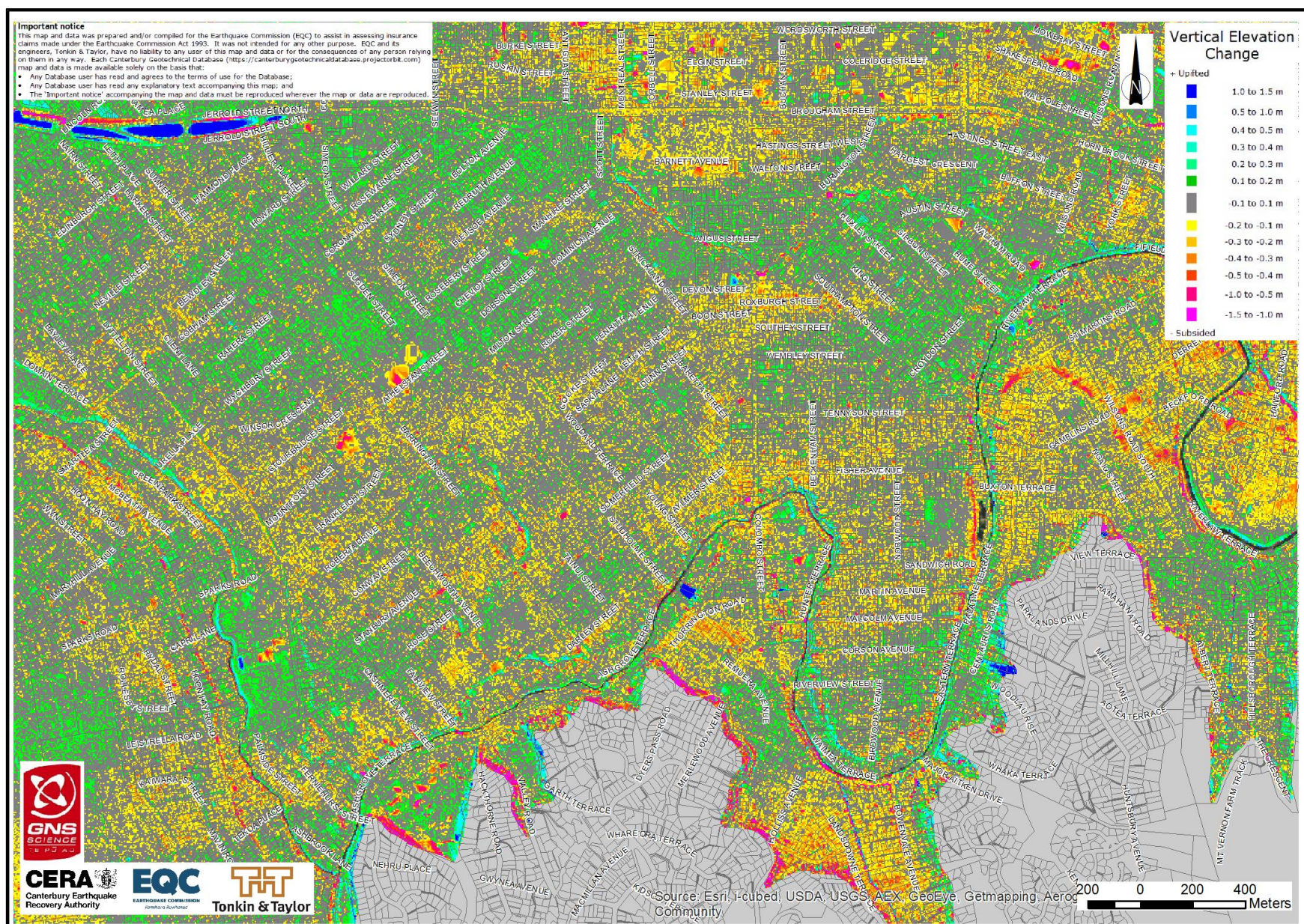
Figure 8 – Change in ground elevation between LiDAR in July 2003 and September 2011 with regional tectonic component of ground displacement removed
