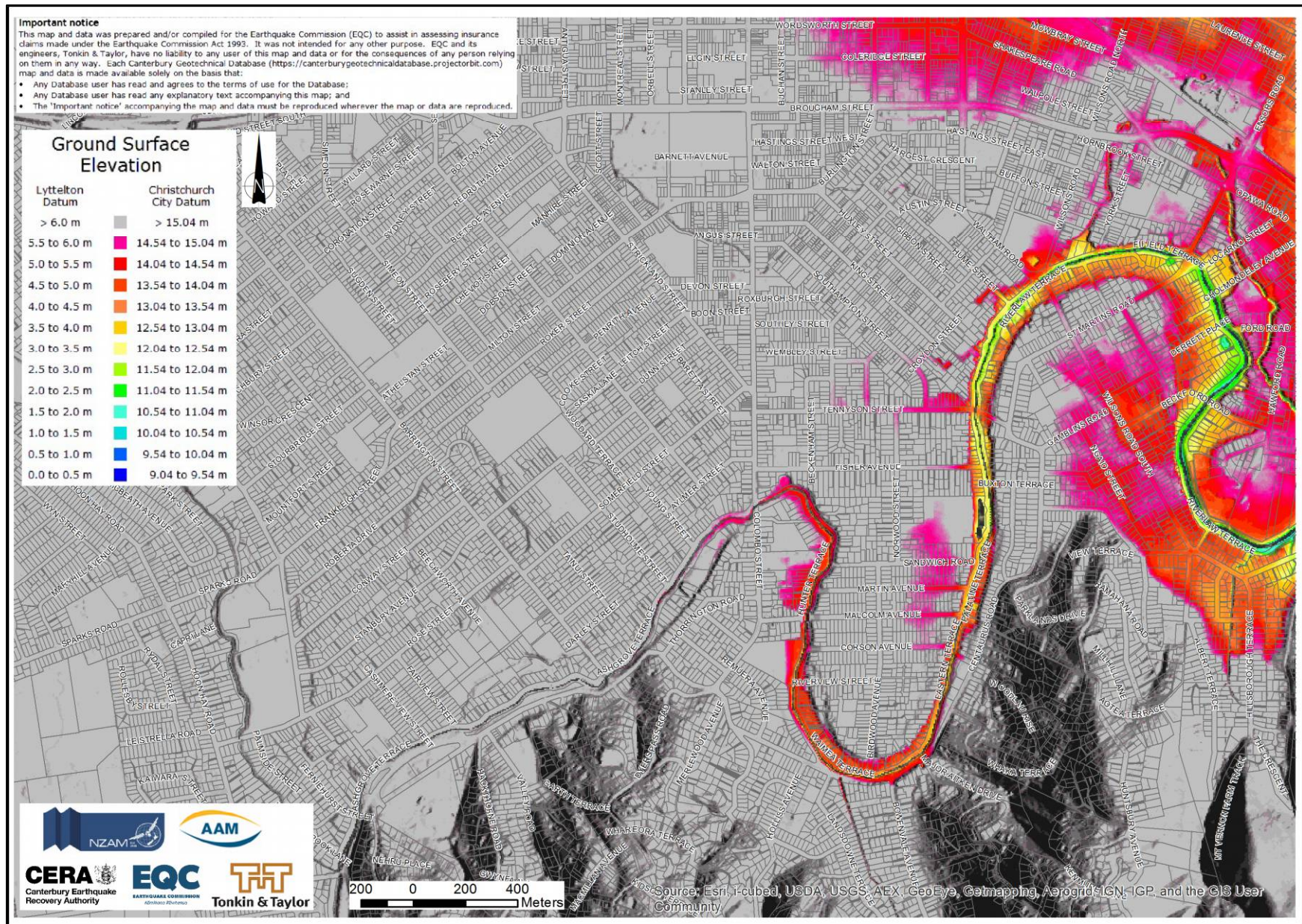
Figure 7 – Ground surface elevation from September 2011 LiDAR survey
